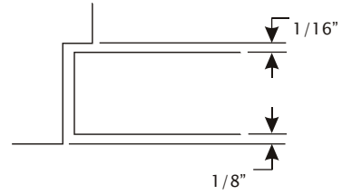
HEAD AND JAMB CLEARANCES
